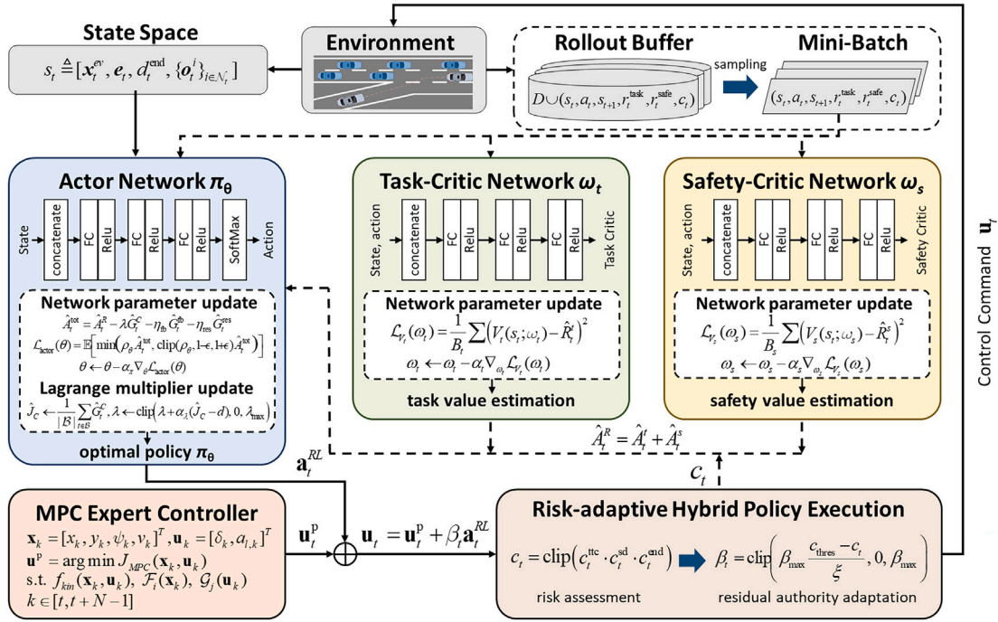
Fig. 3. The policy update process of PR-EPK primarily involves the actor network, task critic and safety critic network, as well as the MPC expert controller and risk-adaptive hybrid policy execution mechanism. The solid line indicates the process of the RL agent interacting with the environment to collect driving experience, while the dashed line represents the parameter updating.
